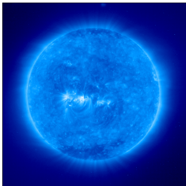
Fe IX,X 171 A
