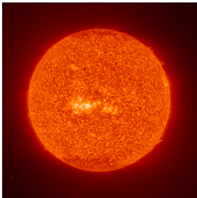
He II 304 A
