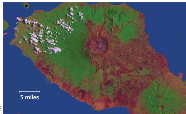
Volcanoes can profoundly influence Earth's climate. This Landsat image shows Tambora, on the Indonesian island of Sumbawa. In April 1815 Tambora unleashed the most powerful volcanic eruption of the past millennium, killing more than 70,000 regional inhabitants and contributing to 1816's "Year Without a Summer."
